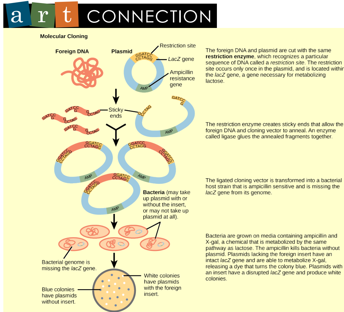
Figure 17.7 This diagram shows the steps involved in molecular cloning.
