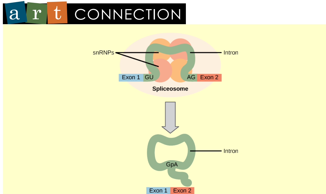
Figure 15.13 Pre-mRNA splicing involves the precise removal of introns from the primary RNA transcript. The splicing process is catalyzed by protein complexes called spliceosomes that are composed of proteins and RNA molecules called snRNAs. Spliceosomes recognize sequences at the 5' and 3' end of the intron.
